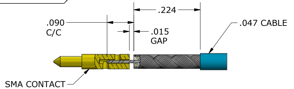
CABLE TRIM VIEW
