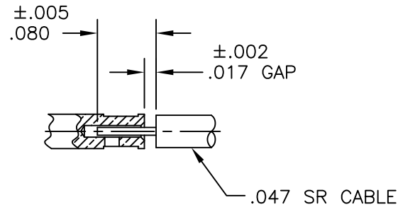
CABLE PREP DETAIL
